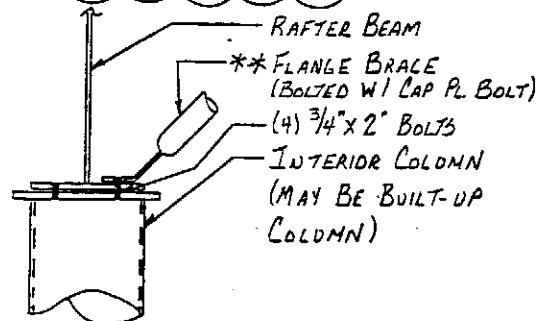
FLANGE BRACE ABOVE INT. COLUMN
